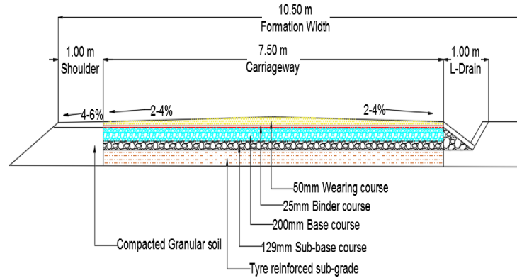
Fig.10 Section of pavement on tyre-reinforced subgrade soil
