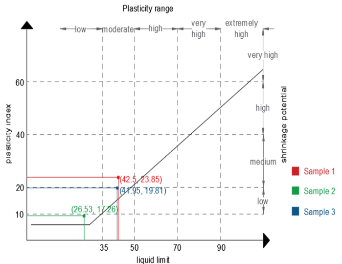
Fig.5 Shrinkage Potential Graph
